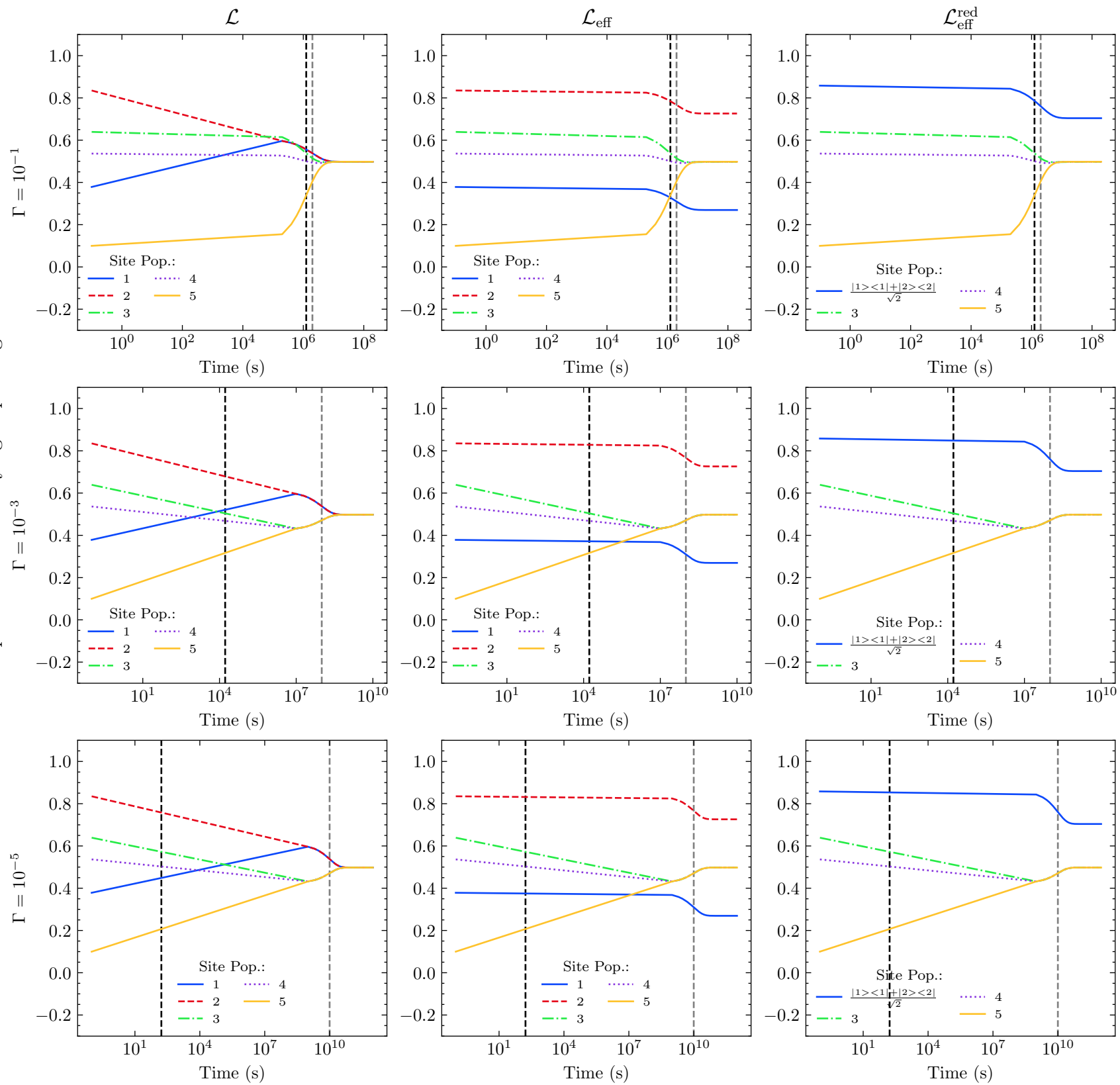
Time Evolution of Site Populations under \mathcal{L} , \mathcal{L}_{\text{eff}} , and \mathcal{L}_{\text{eff}}^{\text{red}} N=5 ; J = 10^{-1} ; \epsilon = 10^{-4}
